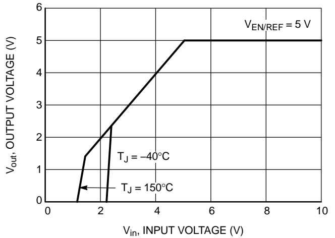
Figure 4. Output Voltage V_{out} vs. Input Voltage V_{in}
