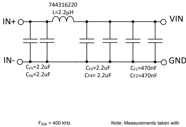
Figure 9-61. Recommended Input EMI Filter
