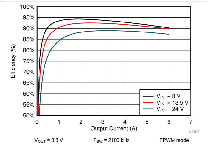
Figure 9-10. LM61460 Efficiency
