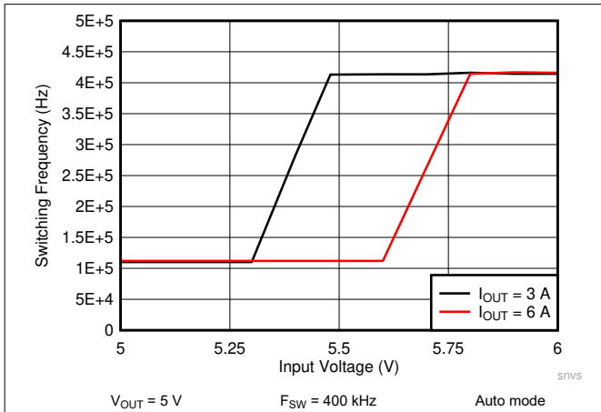
Figure 9-35. LM61460 Frequency Dropout Curve
