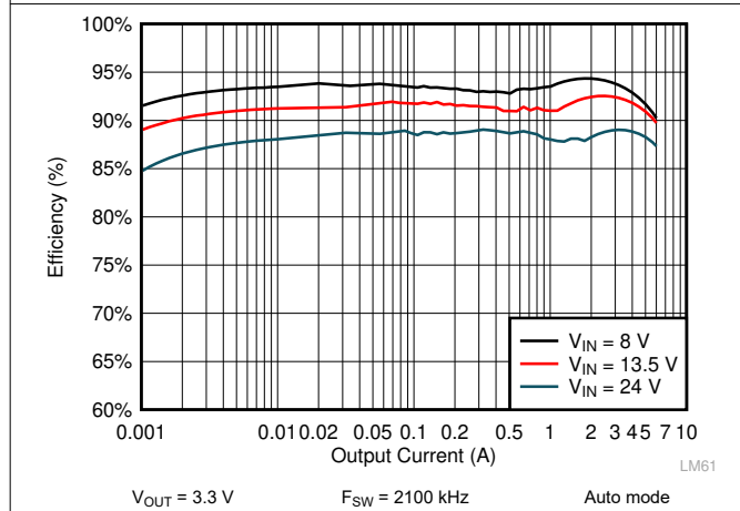
Figure 9-9. LM61460 Efficiency
