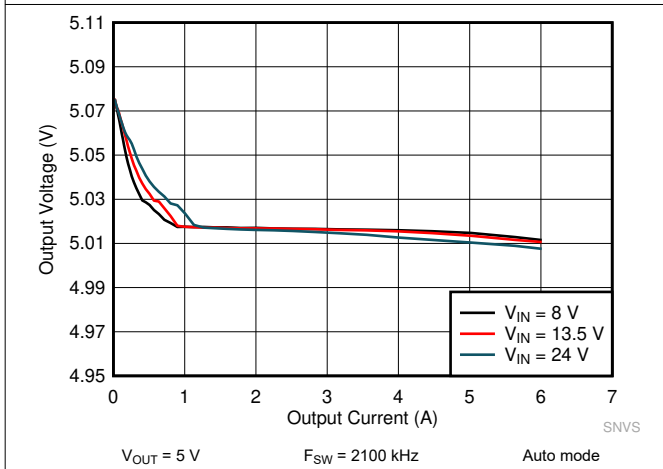
Figure 9-27. LM61460 Load and Line Regulation
