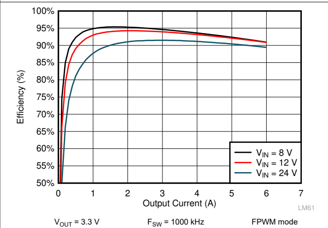
Figure 9-8. LM61460 Efficiency
