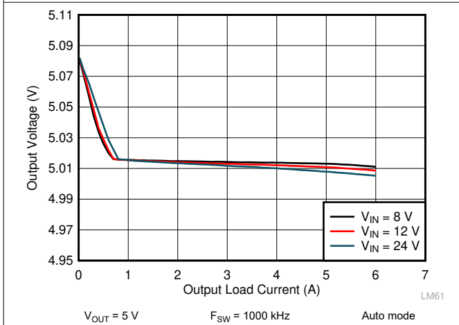
Figure 9-25. LM61460 Load and Line Regulation
