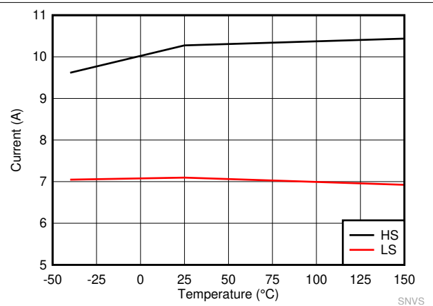
Figure 7-4. LM61460 High-Side and Low-Side Current Limits
