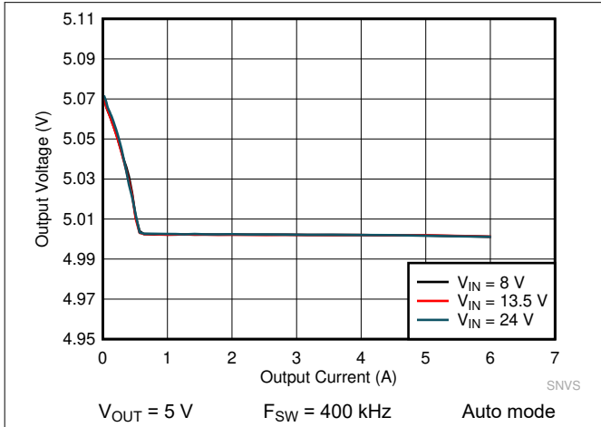
Figure 9-23. LM61460 Load and Line Regulation
