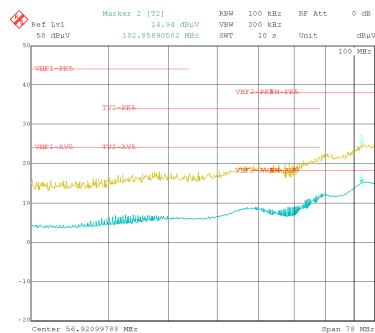
Figure 9-55. Conducted EMI versus CISPR25 Limits (Yellow: Peak Signal, Blue: Average Signal)
