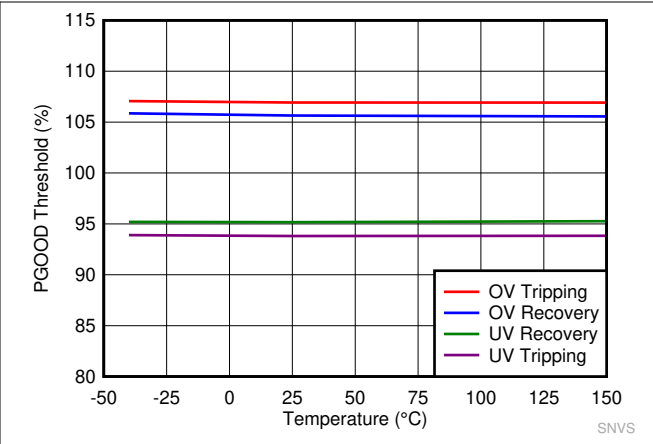
Figure 7-8. PGOOD Thresholds
