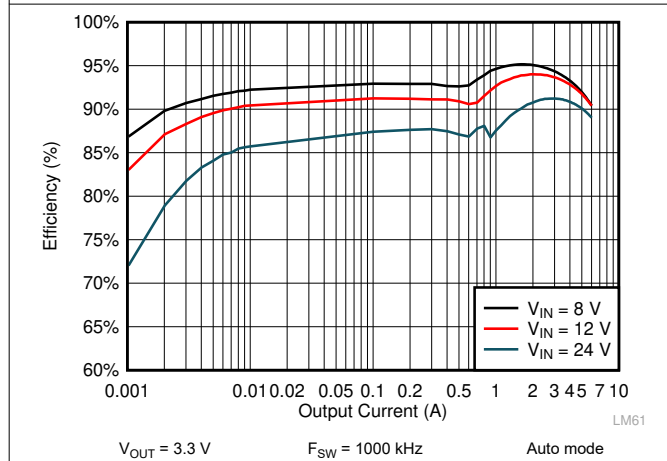
Figure 9-7. LM61460 Efficiency
