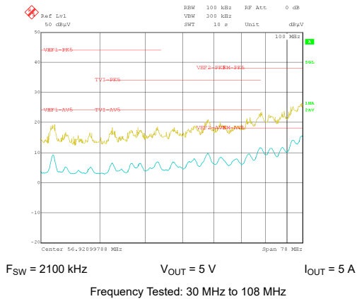
Figure 9-63. Conducted EMI versus CISPR25 Limits (Yellow: Peak Signal, Blue: Average Signal)
