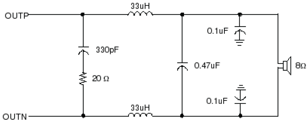
Figure 57. Typical LC filter for an 4 Ω speaker
