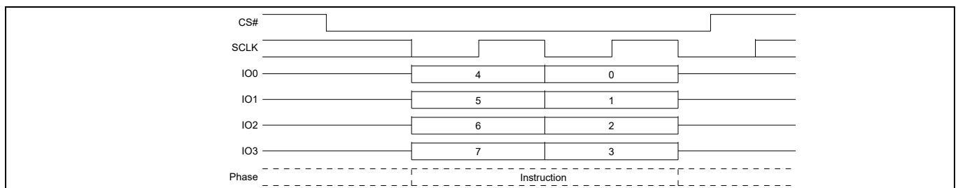
Figure 85 Erase or Program Suspend command sequence QPI mode
