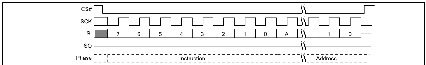
Figure 81 EES command sequence [56]
