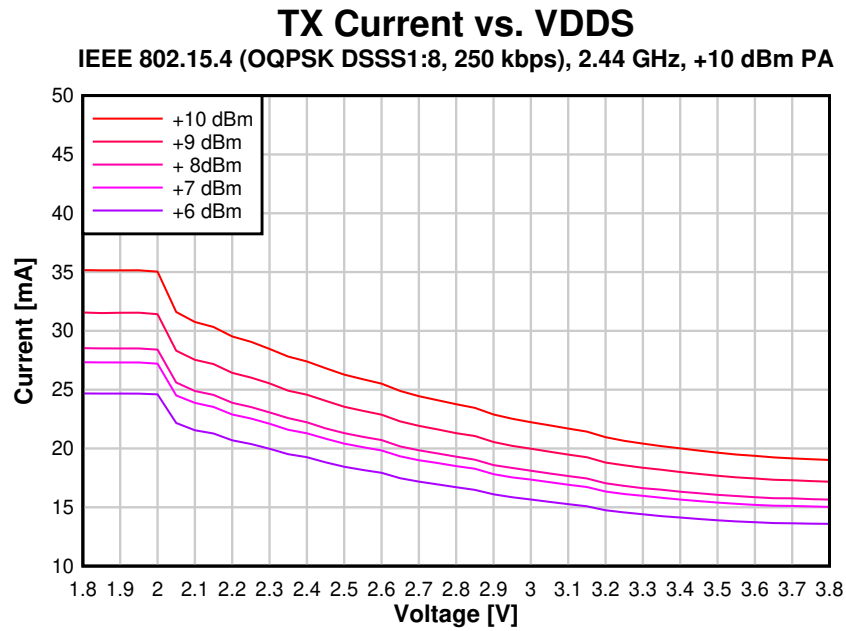
Figure 8-13. TX Current vs. Supply Voltage (VDDS) (250 kbps, 2.44 GHz, +10 dBm PA)
