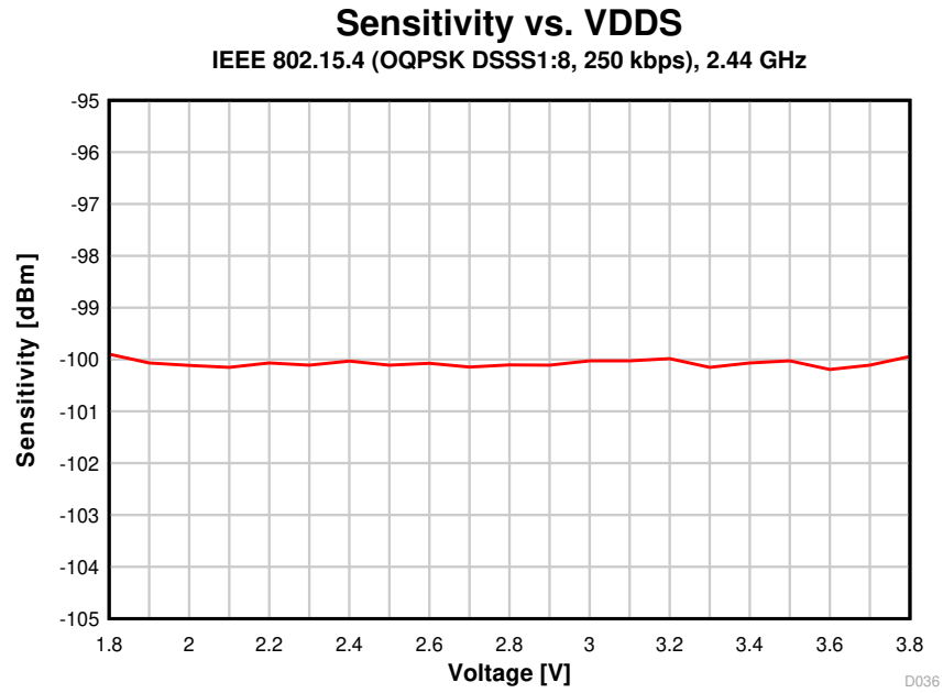
Figure 8-20. Sensitivity vs. Supply Voltage (VDD5) (250 kbps, 2.44 GHz)
