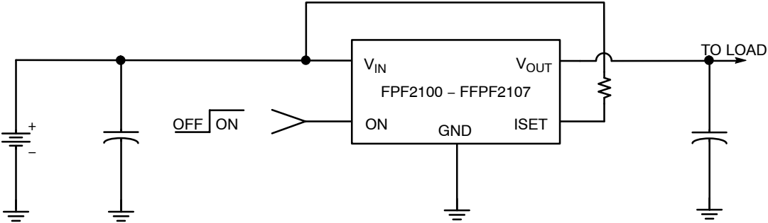
Figure 1. Typical Application
